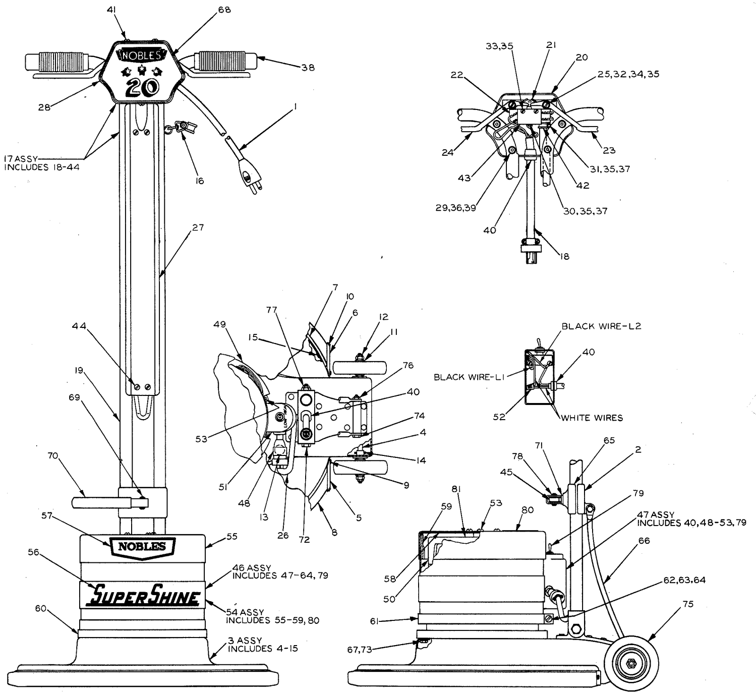
PARTS BREAKDOWN — MODEL 202
